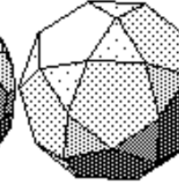
Icosidodecahedron
