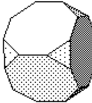
Truncated Cube
