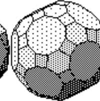
(Rhombi)truncated Icosidodecahedron
