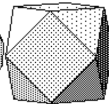
Cuboctahedron (Dymaxion)
