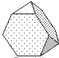
Truncated Tetrahedron
